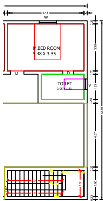
FLOOR PLAN
