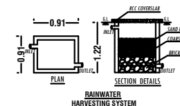
RAINWATER HARVESTING SYSTEM
