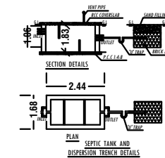
SECTION DETAILS
