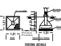
FOOTING DETAILS
