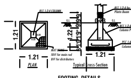
FOOTING DETAILS
