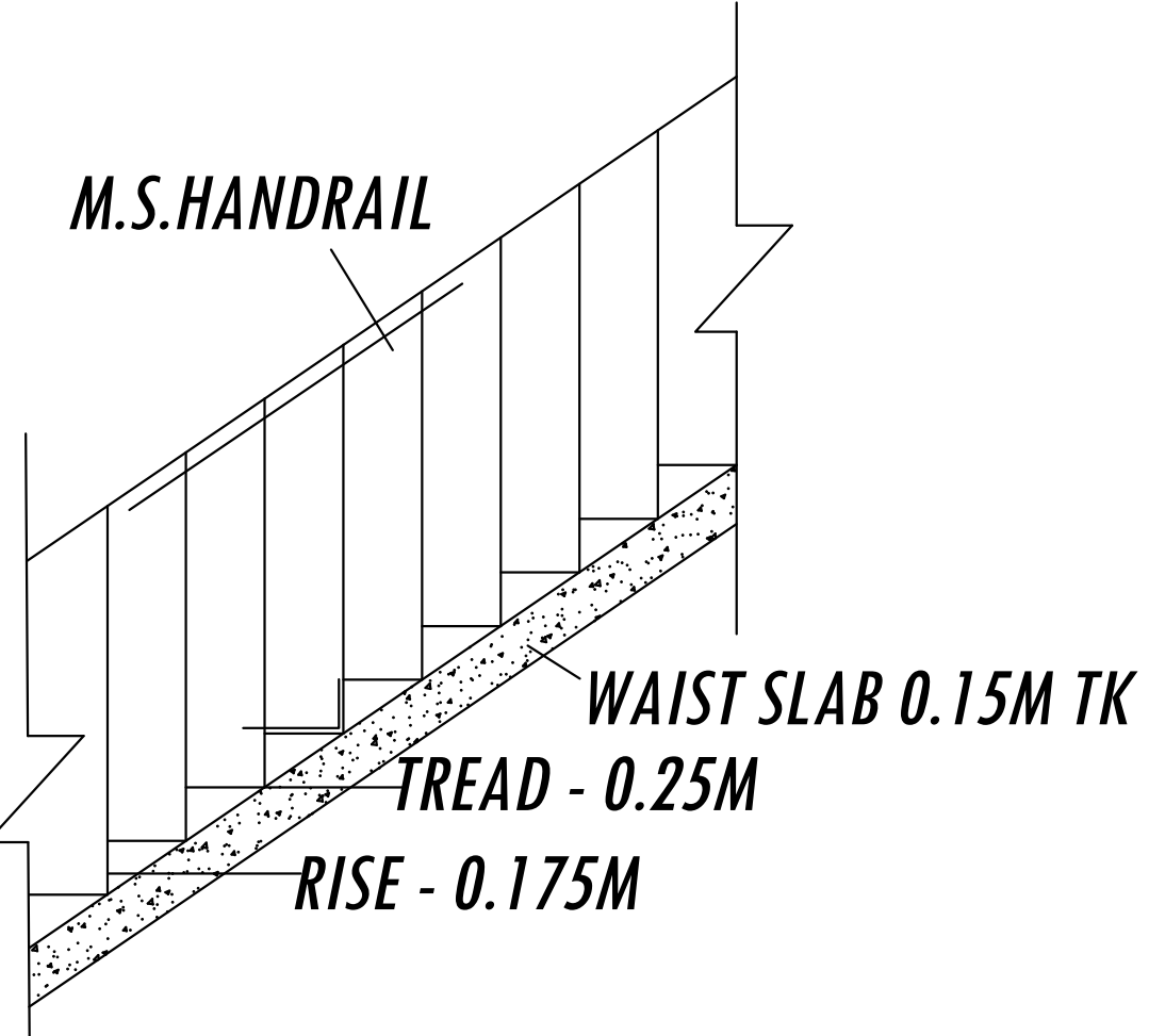
STAIR CASE DETAILS
