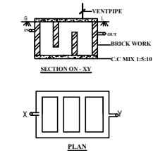
SEPTICTANK DETAILS
