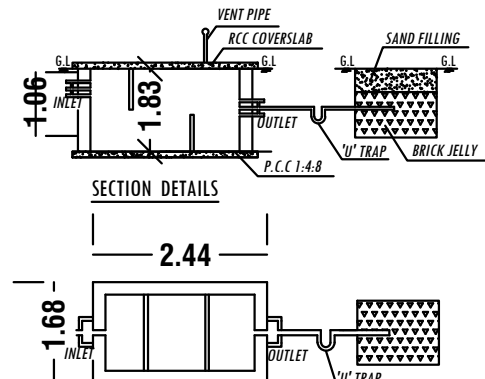
PLAN SEPTIC TANK AND DISPERSION TRENCH DETAILS
