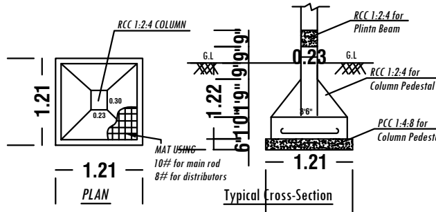
FOOTING DETAILS
