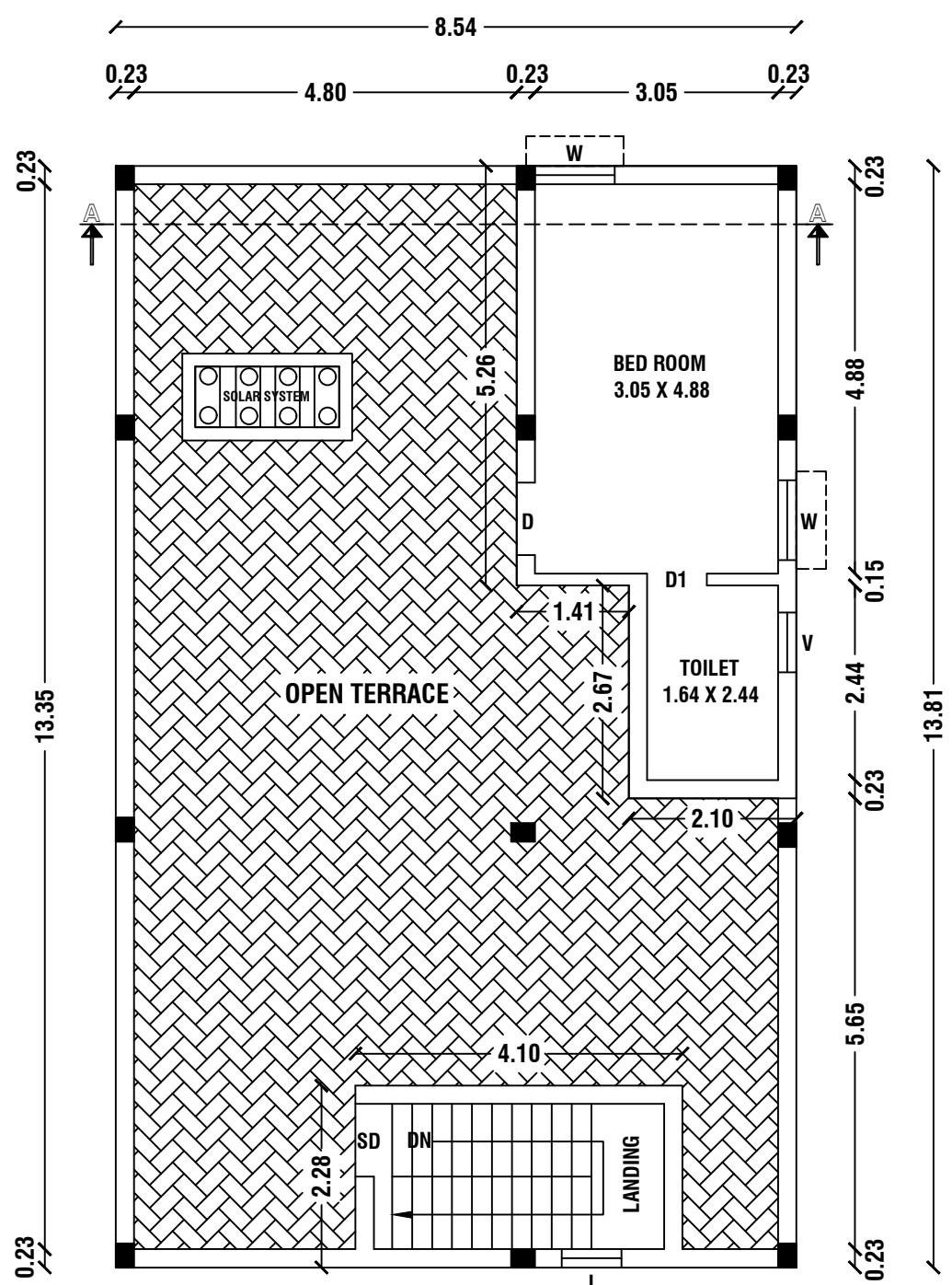
FIRST FLOOR PLAN CUM OPEN TERRACE FLOOR PLAN
