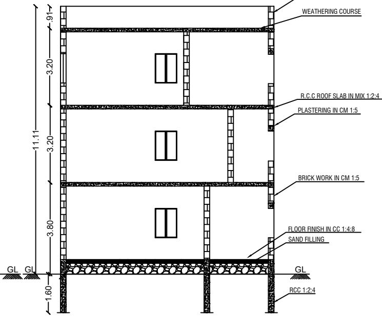
SECTION ON "MA"
