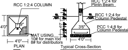
TYPICAL CROSS-SECTION
