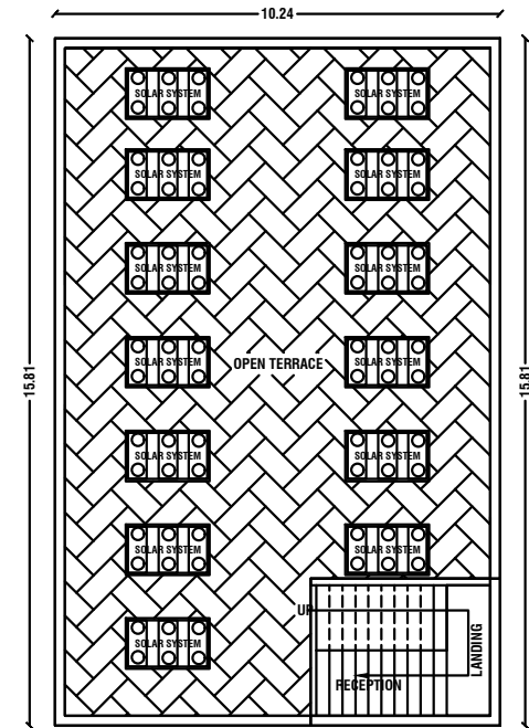
OPEN TERRACE FLOOR PLAN
