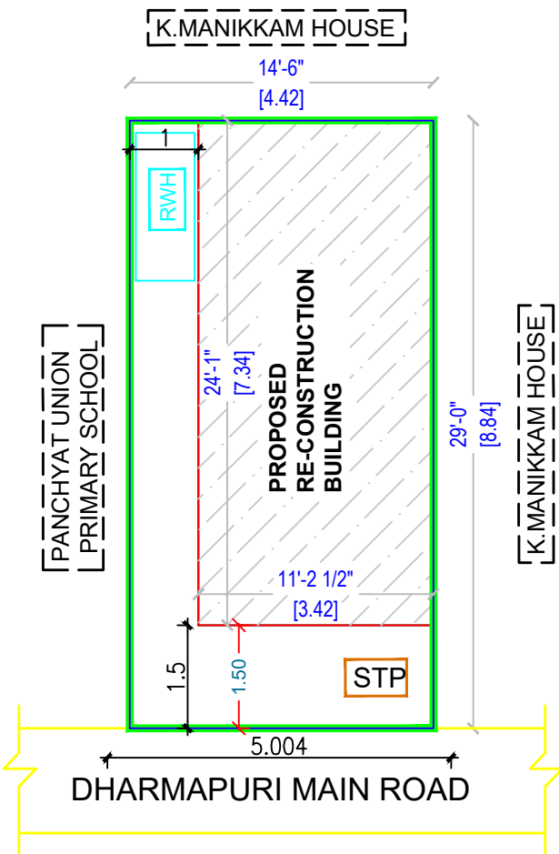
SITE PLAN FOR PROPOSED BUILDING
