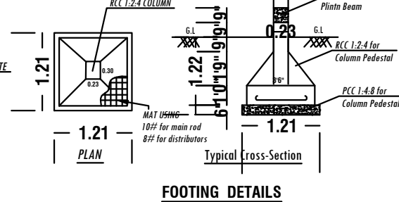
FOOTING DETAILS
