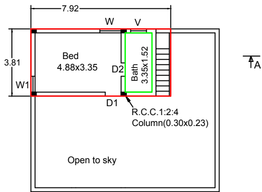
PLAN - First Floor
