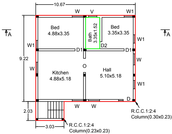
PLAN - Ground Floor
