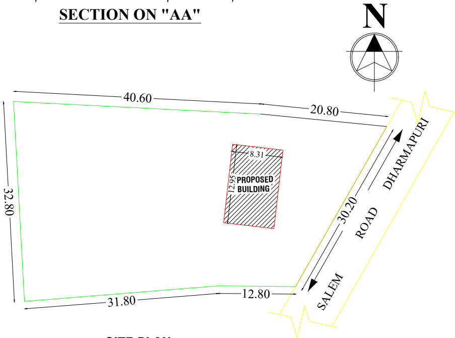
SITE PLAN
