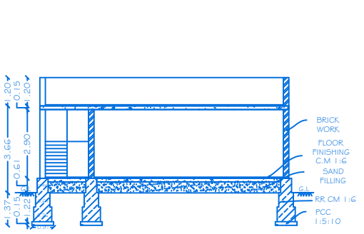
SECTION ON-AA
