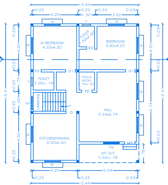
BLOCK 2 GROUND FLOOR PLAN
