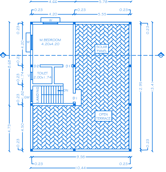
BLOCK 2 FIRST FLOOR PLAN
