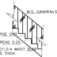
STAIRCASE DETAILS SCALE- 1:20
