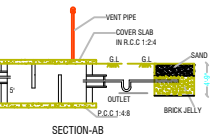
SECTION-A-B
