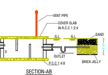
SECTION-A-B
