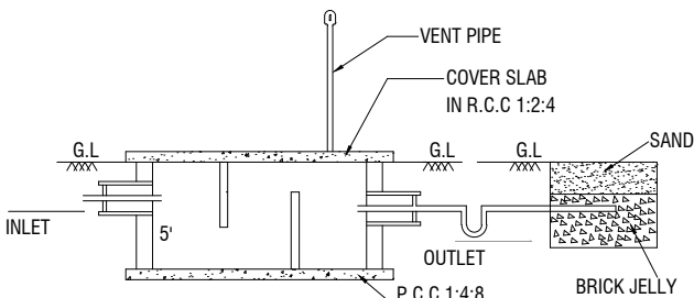
SECTION-AB
