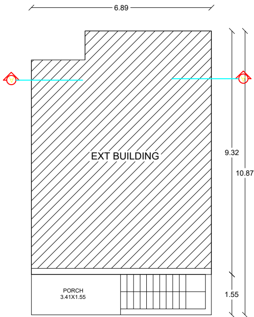
EXT & PRO GROUND FLOOR
