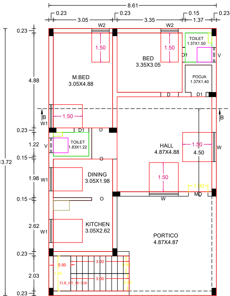
BLOCK -2 GROUND FLOOR PLAN
