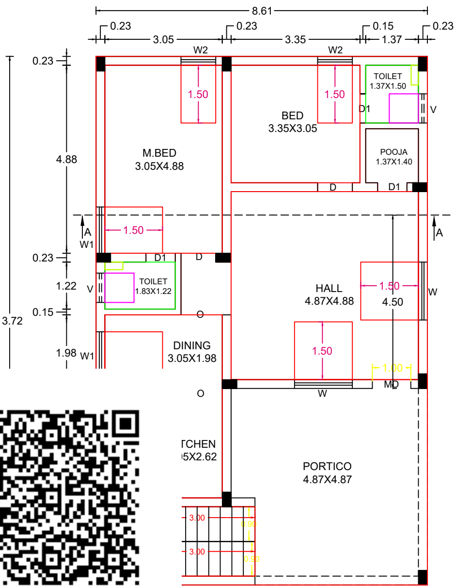
BLOCK-1 GROUND FLOOR PLAN
