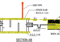
SECTION-AB
