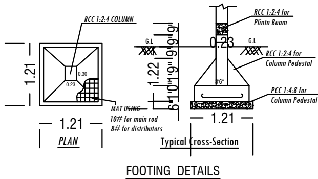
FOOTING DETAILS
