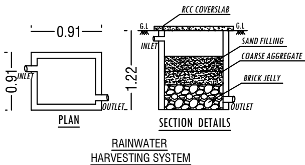
RAINWATER HARVESTING SYSTEM
