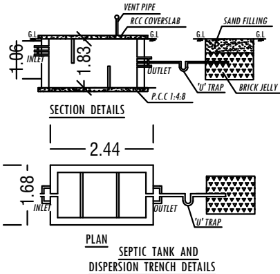
SEPTIC TANK AND DISPERSION TRENCH DETAILS
