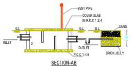
SECTION-AB
