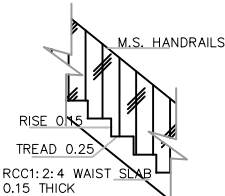
STAIRCASE DETAILS SCALE- 1:20
