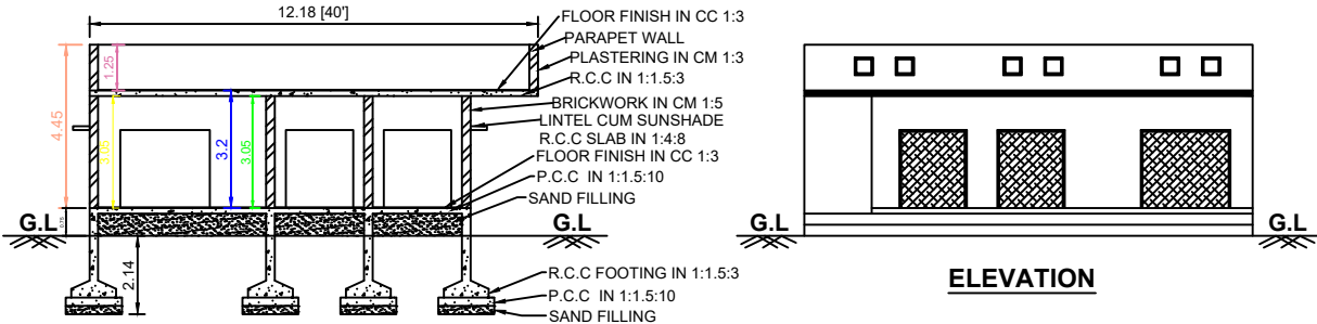
SECTION ON AB
