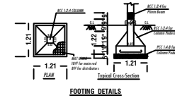
FOOTING DETAILS
