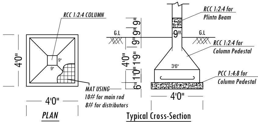
FOOTING DETAILS
