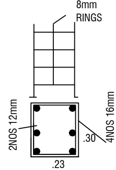
COLUMN DETAILS
