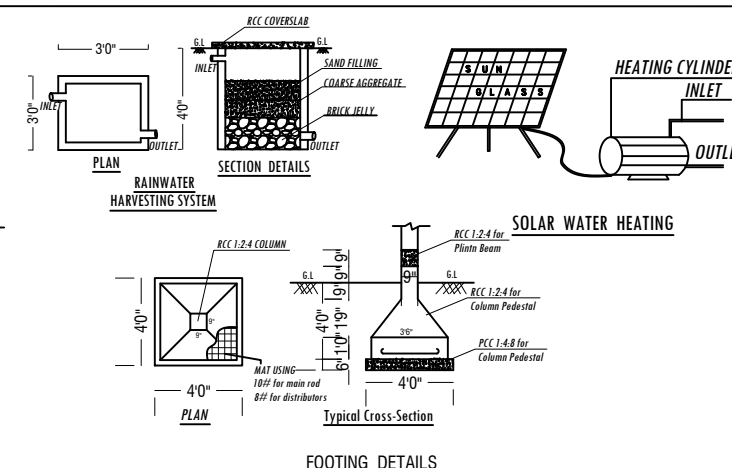
FOOTING DETAILS
