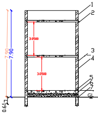
SECTION - "AAA"
