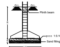
FOUNDATION DETAILS
