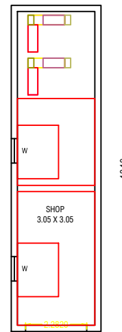
GROUND FLOOR PLAN
