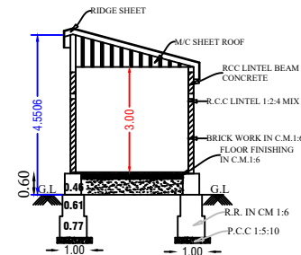
SECTION ON-"AB"
