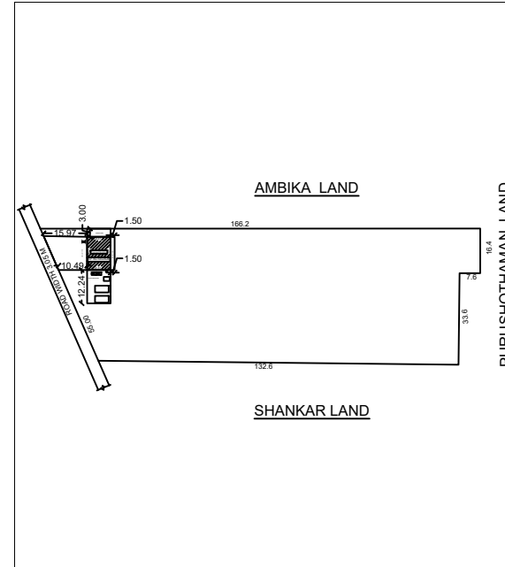
SITE PLAN SCALE 1:200 & As Per FMB
