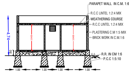
SECTION ON-"AB"
