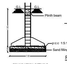
FOUNDATION DETAILS
