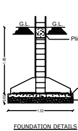
FOUNDATION DETAILS
