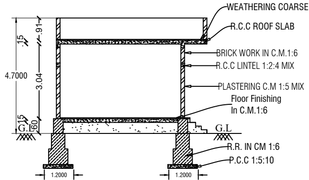
SECTION ON-"AB"
