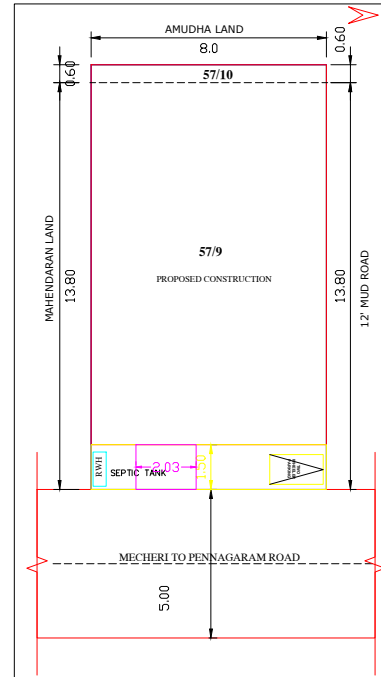
TOPO PLAN
