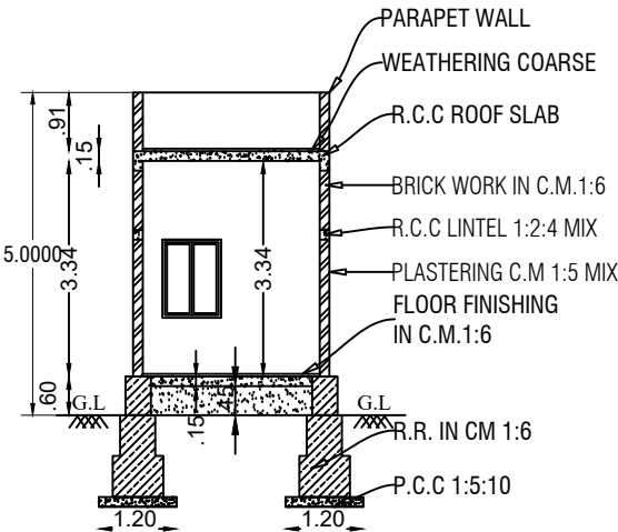
SECTION ON-"AB"
