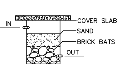
RAINWATER HARVEST NOT TO SCALE
