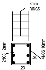
COLUMN DETAILS (NOT TO SCALE)
