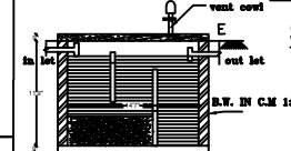
SECTIONAL ELEVATION
