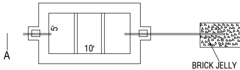
SEPTIC TANK & DISPERSION TRENCH DETAILS SCALE- 1:100
