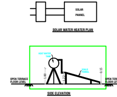
SIDE ELEVATION
