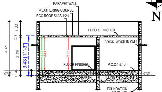
SECTION "A-B"
