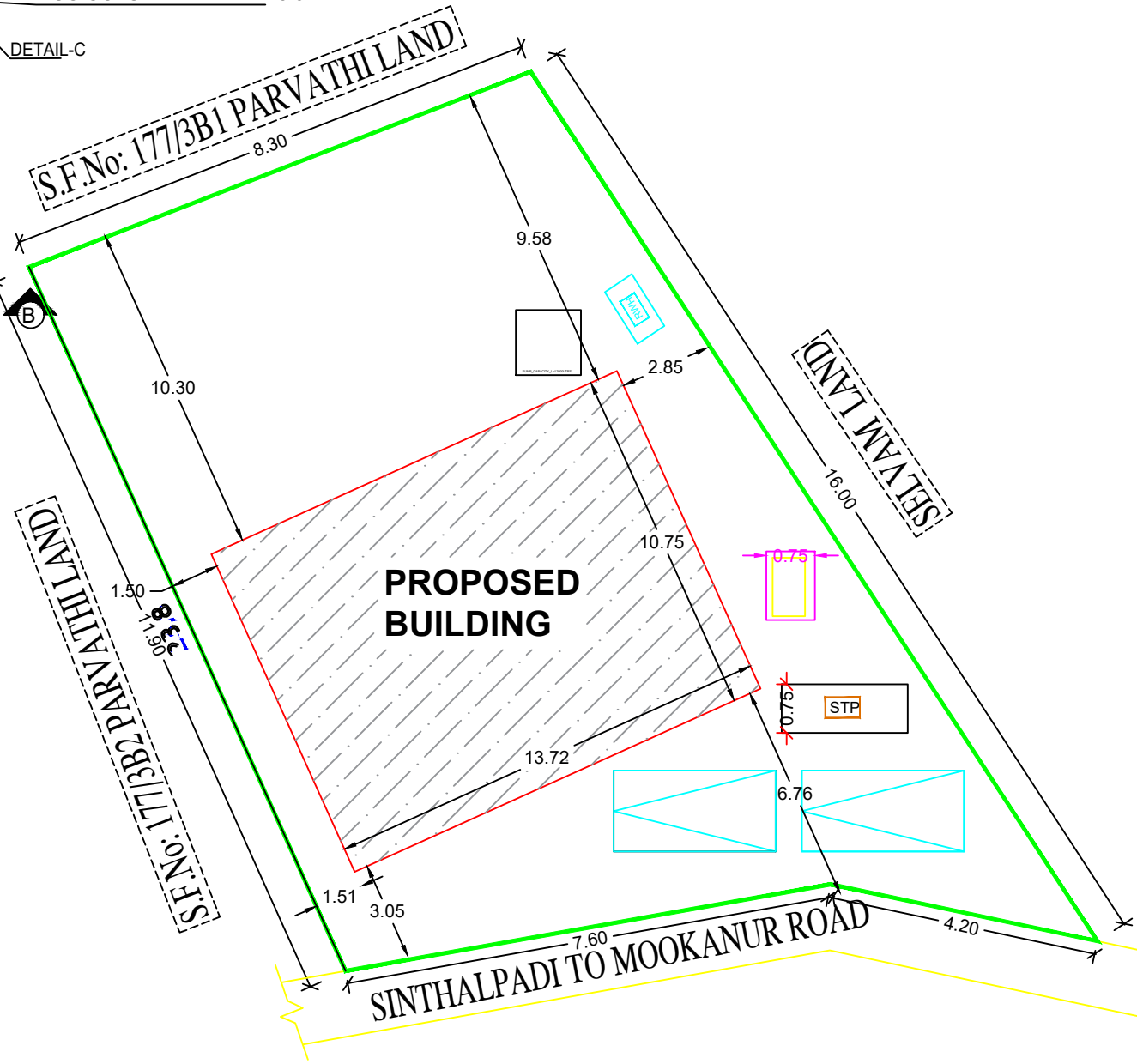
SITE PLAN
