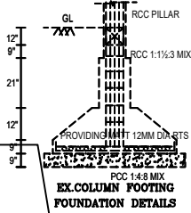
FOUNDATION DETAILS
