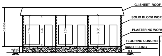
SECTION- AB
