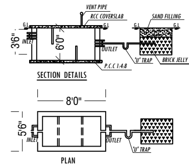
SEPTIC TANK AND DISPERSION TRENCH DETAILS
