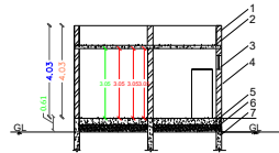
SECTION ON 'AA'
