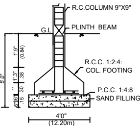
FOUNDATION DEATAILS
