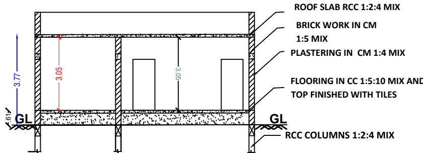
SECTION ON-AA'
