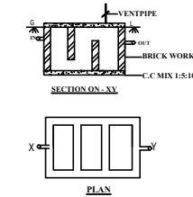
SEPTICTANK DETAILS
