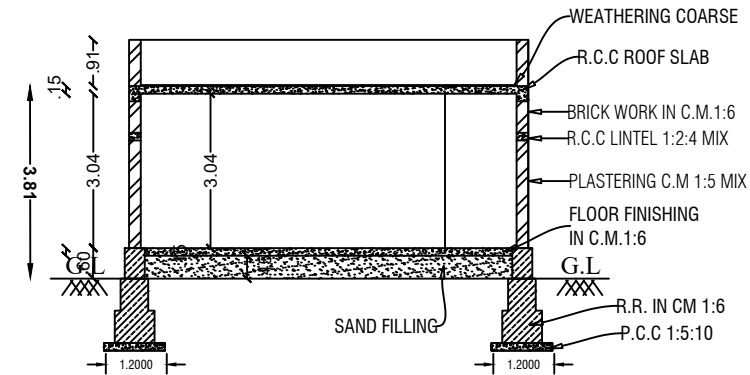
SECTION ON-"AB"
