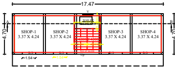
GROUND FLOOR PLAN
