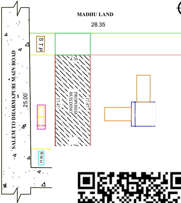
SITE PLAN
