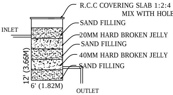
WASTE WATER RECYCLE UNIT
