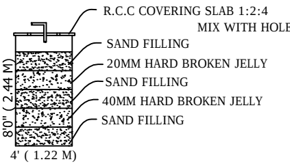
RAIN WATER HARVEST UNIT
