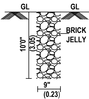
PERCULATION PIT
