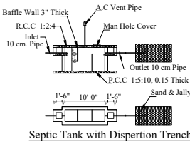
Septic Tank with Dispersion Trench
