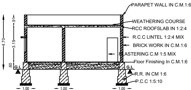
SECTION ON-'AB'
