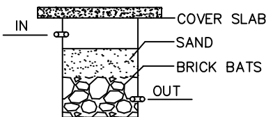
SECTION
