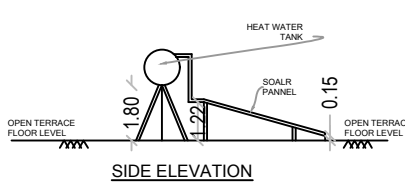
SOLAR WATER HEATER SCALE- 1:50
