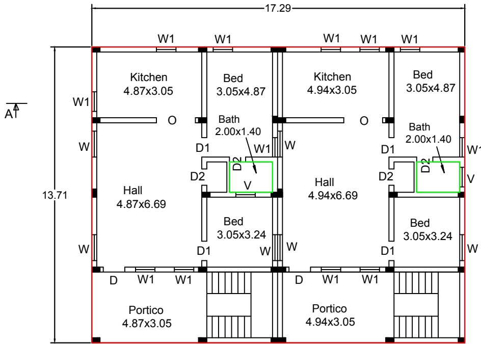
PLAN - Ground Floor
