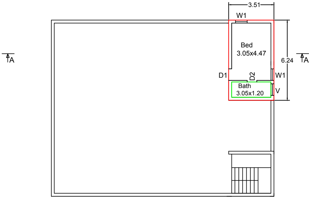
PLAN - Second Floor
