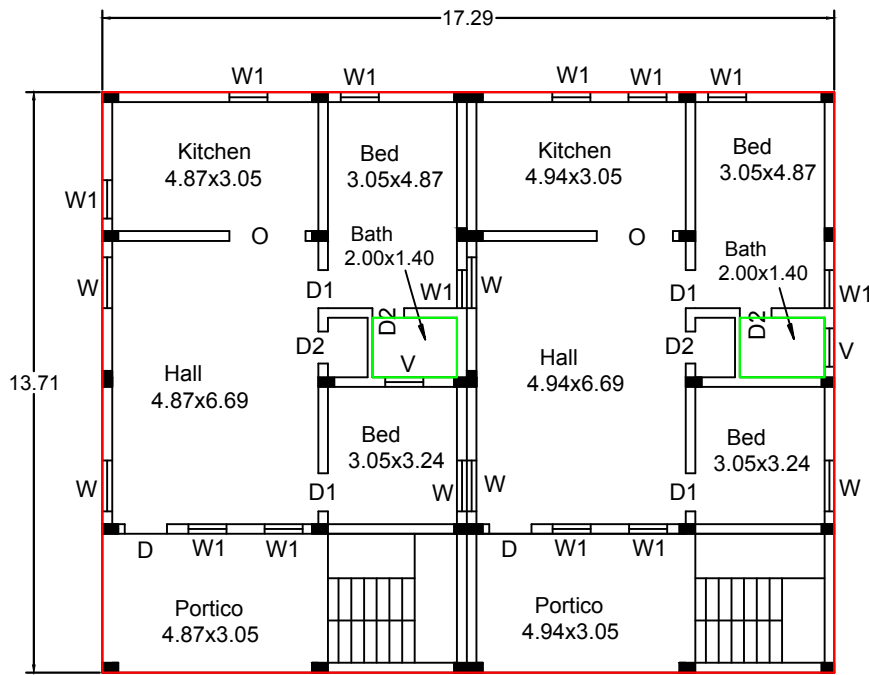
PLAN - First Floor
