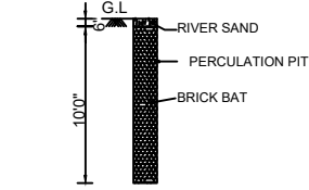
PERCOLATION PIT
