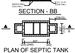
PLAN OF SEPTIC TANK
