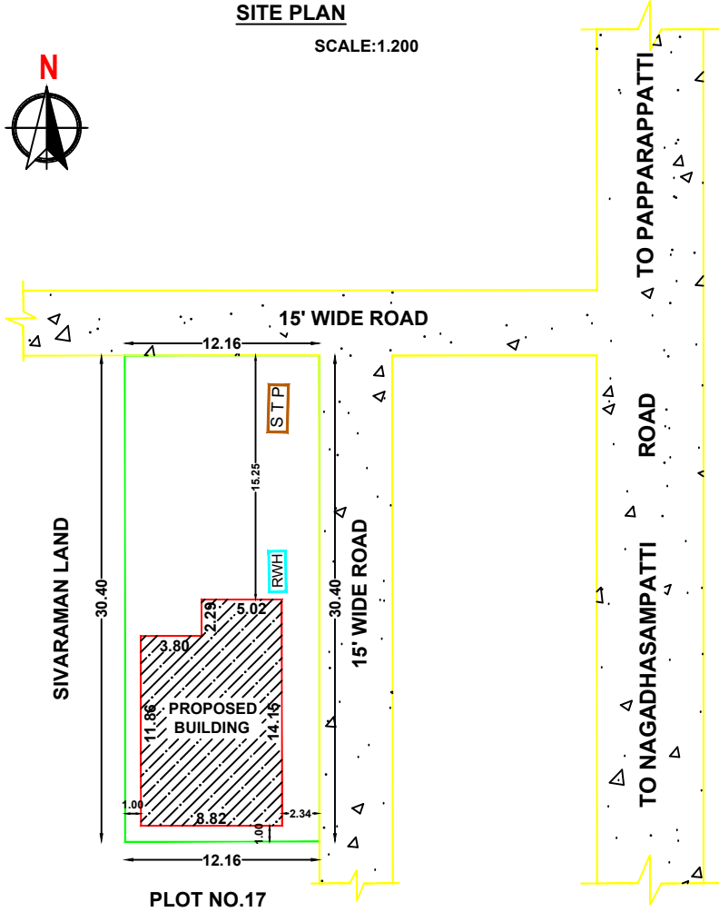
PLOT NO.17
