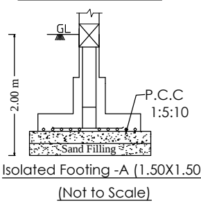
FOUNDATION DETAIL - A
